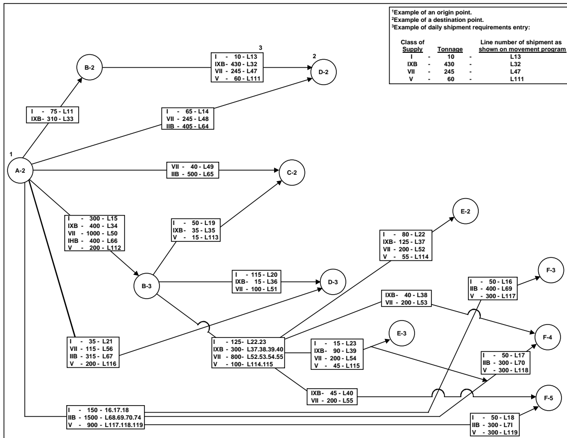
Figure 7-6. Requirements Schematic
